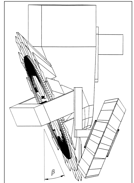
Fig. 2: Side view of revolving spade planter (indication of vertical decline angle β)
